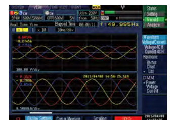
Voltage and current of spot welding machine after treatment
